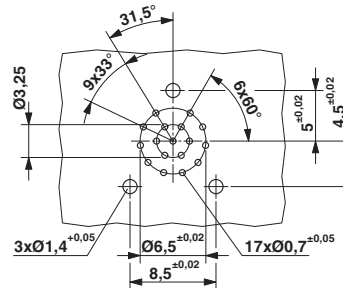
Drilling diagram
